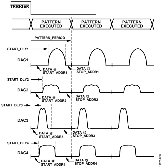
Figure 50. Pattern Using Different Waveforms Stored in SRAM
