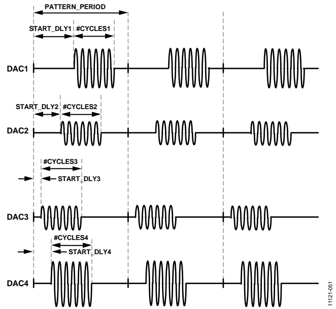
Figure 51. Pulsed Sine Waves in Pattern Periods
