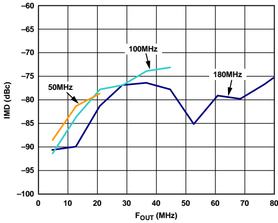
Figure 25. IMD vs. F_{OUT} , Three F_{OUT} Values
