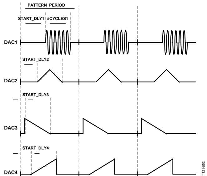
Figure 52. Pulsed SineWaves and Sawtooth Waveforms in Pattern Periods
