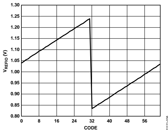
Figure 38. Typical V_{REFIO} Voltage vs. BGDR
