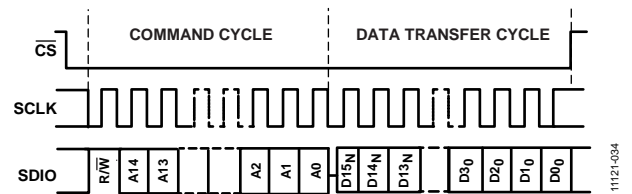
Figure 34. Serial Register Interface Timing, MSB First Read, 3-Wire SPI
