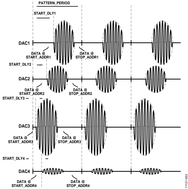
Figure 53. DDS Output Amplitude Modulated by RAM Envelope
