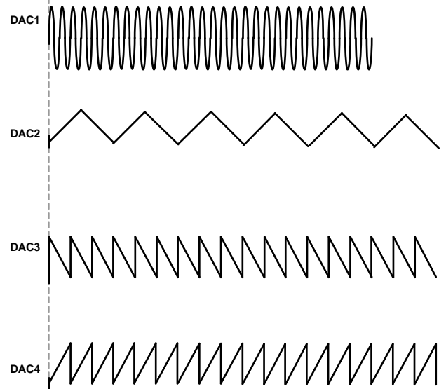
Figure 55. Waveforms Without Start Delays
