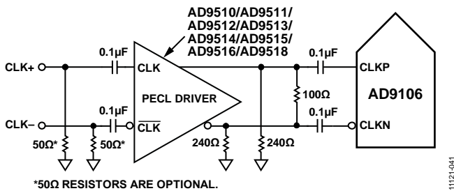
Figure 41. Differential PECL Sample Clock
