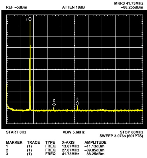
Figure 24. Output Spectrum F_{OUT} = 13.87 MHz
