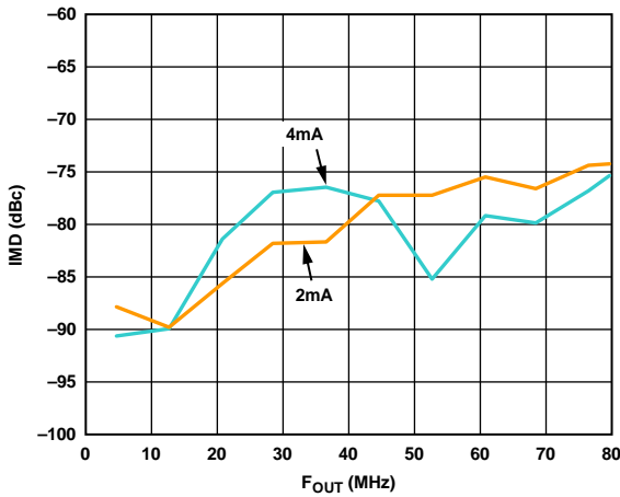
Figure 26. IMD vs. F_{OUT} , Two I_{OUTFS} Values
