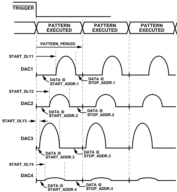
Figure 43. Periodic Pulse Trains output on all DACx
