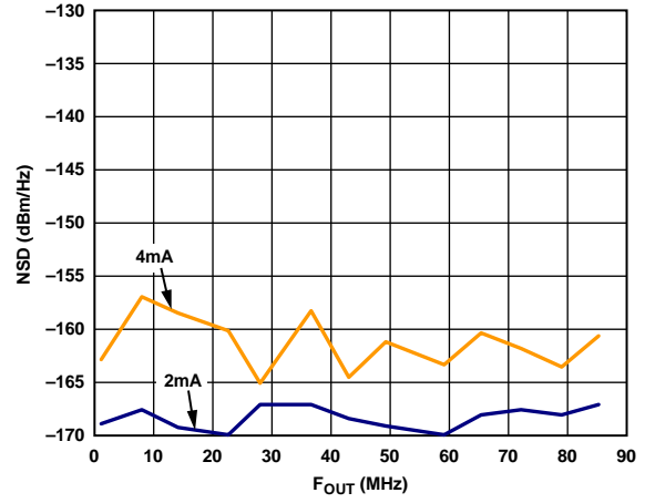
Figure 28. NSD vs. F_{OUT} , Two I_{OUTFS} Values
