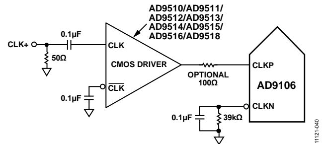
Figure 40. Single-Ended 1.8 V CMOS Sample Clock
