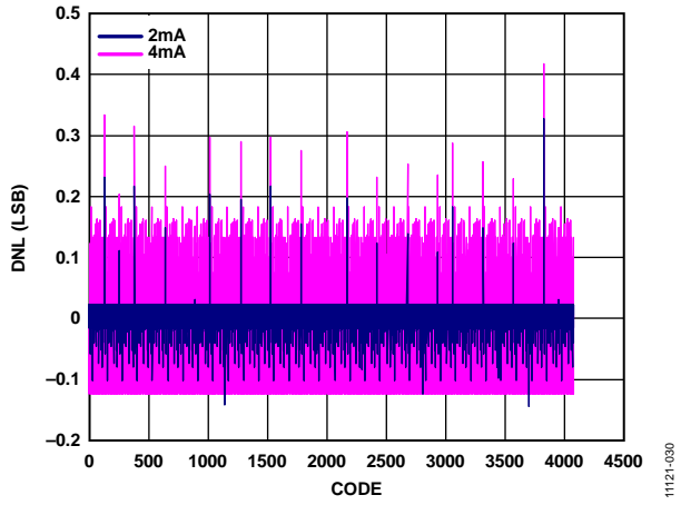
Figure 30. DNL, Three I_{OUTFS} Values
