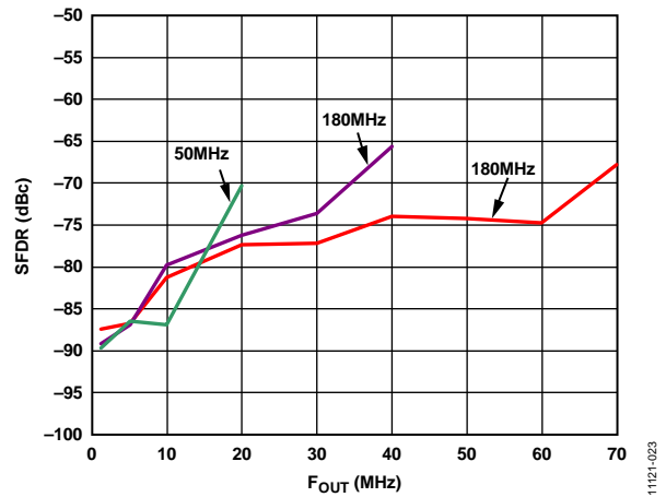
Figure 23. SFDR at Three F_{DAC} vs. F_{OUT}
