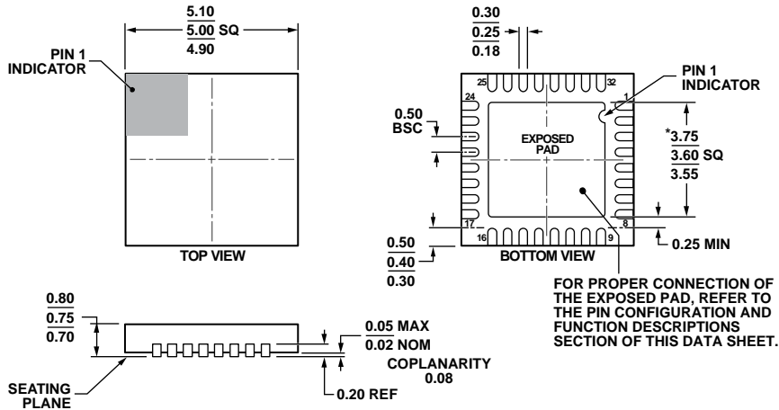
Figure 56. 32-Lead Lead Frame Chip Scale Package [LFCSP_WQ] 5 mm × 5 mm Body, Very Very Thin Quad (CP-32-12) Dimensions shown in millimeters
