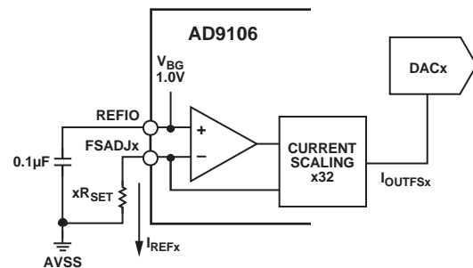
Figure 37. On-Chip Reference with External xR_{SET} Resistor
