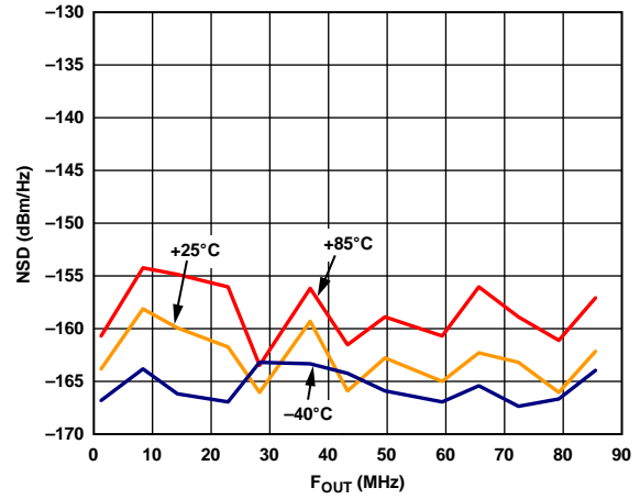
Figure 29. NSD vs. F_{OUT} at Three Temperatures
