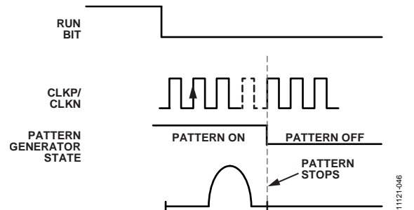
Figure 46. RUN Bit Driven Pattern Stop
