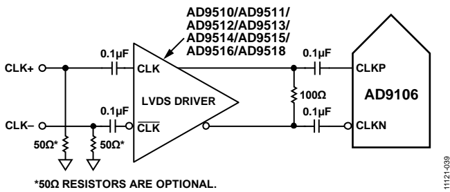
Figure 39. Differential LVDS Clock Input
