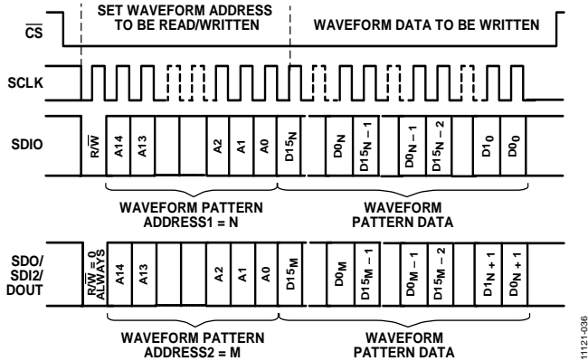
Figure 36. Double SPI Write of SRAM Data
