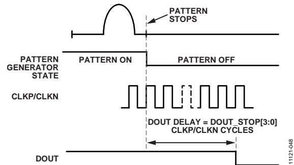
Figure 48. DOOUT Stop Sequence
