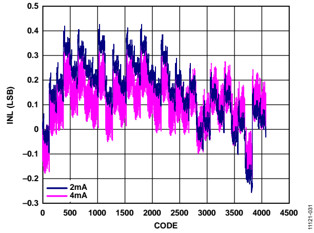
Figure 31. INL, Two I_{OUTFS} Values
