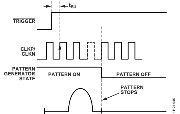
Figure 45. Trigger Rising Edge Initiated Pattern Stop
