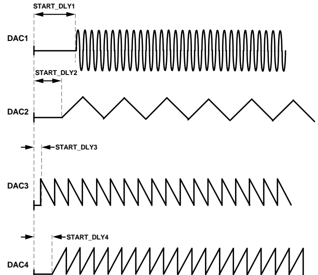
Figure 54. Waveforms with Start Delays
