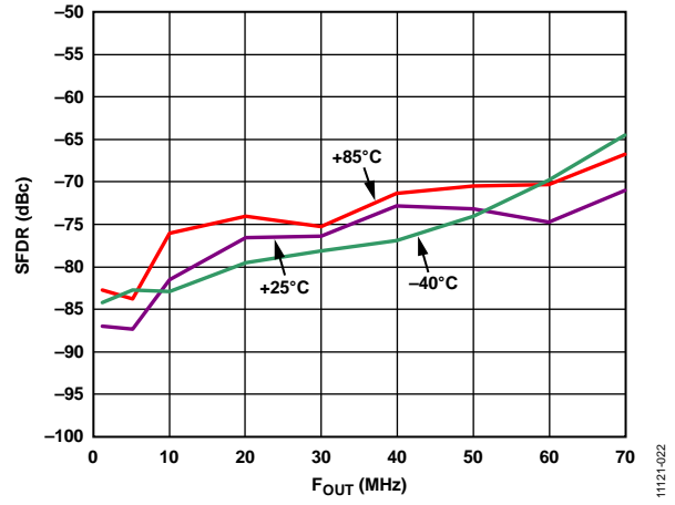
Figure 22. SFDR at Three Temperatures vs. F_{OUT}
