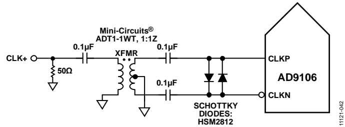
Figure 42. Transformer Coupled Clock
