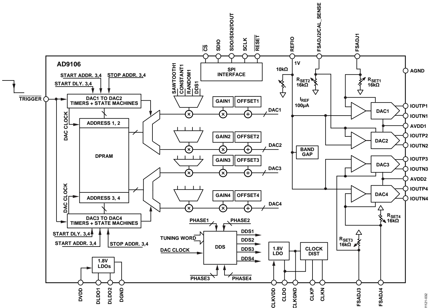
Figure 32. AD9106 Block Diagram
