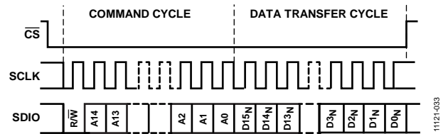
Figure 33. Serial Register Interface Timing, MSB First Write, 3-Wire SPI
