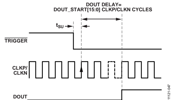
Figure 47. DOOUT Start Sequence
