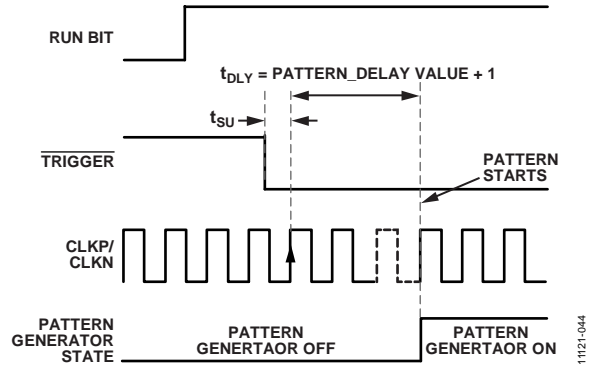
Figure 44. Trigger Initiated Pattern Start with Pattern Delay
