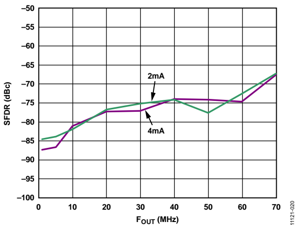
Figure 20. SFDR at Two I_{OUTFS} vs. F_{OUT}
