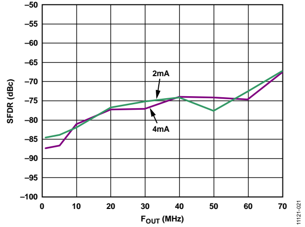
Figure 21. SFDR at Two I_{OUTFS} vs. F_{OUT}
